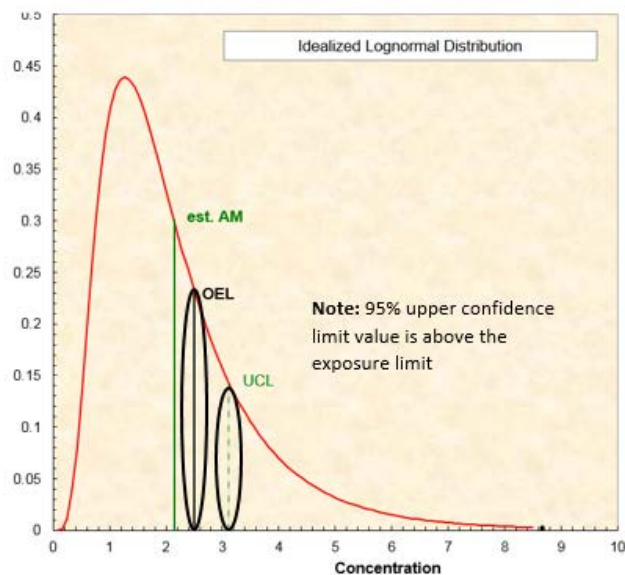
Figure 2: Example dataset—non-conforming
