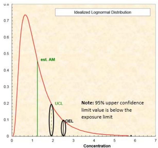
Figure 3: Example dataset—conforming
